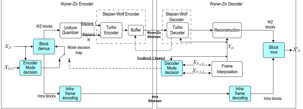
Fig. 1. IST-PDWZ video codec architecture
