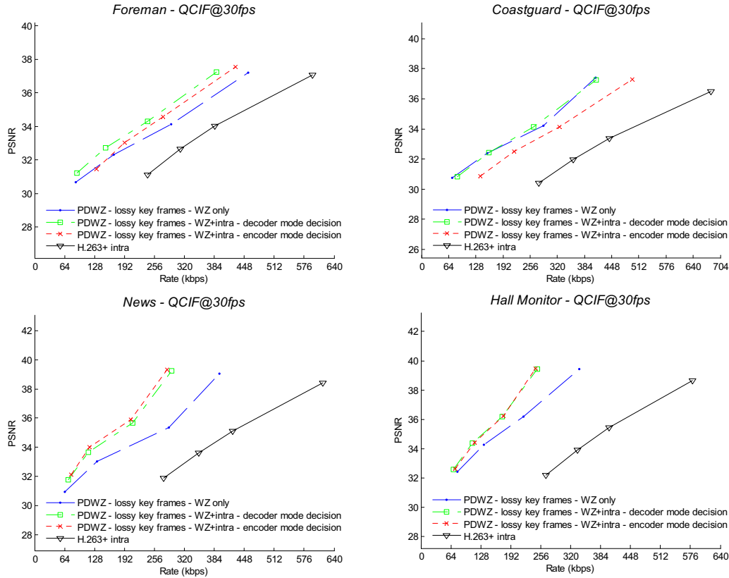
Fig. 2. IST-PDWZ rate-distortion curves: intra-mode decision at the encoder vs. at the decoder
