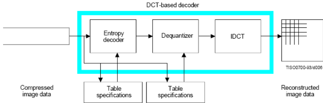
Figure 2– DCT based JPEG decoder.
