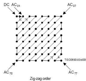
Figure 3 – Zig-zag scanning order.
