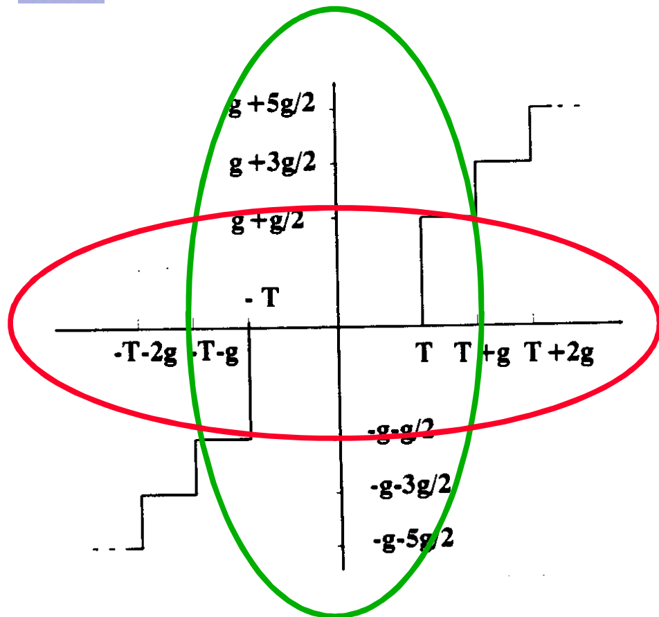
Example quantization characteristic
